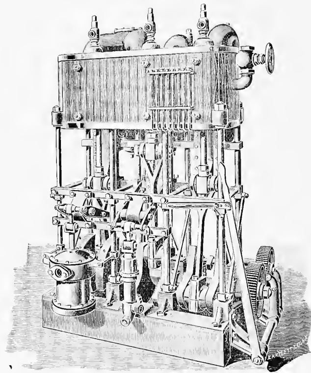
THE SEABURY TRIPLE-EXPANSION YACHT ENGINE.
